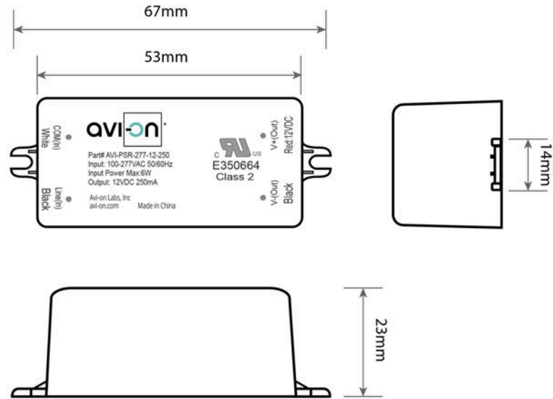
Figure 1. Dimensions
